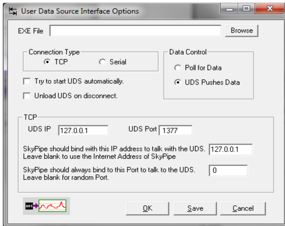
Illustration 37: UDS configuration window in Radio-SkyPipe.
