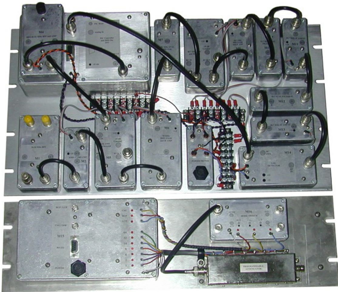
Illustration 40: FS200B production model spectrograph with an automated step calibrator on the bottom panel. Everything can be controlled remotely via the serial port attached PC. From the front of the rack you just see an led, reset button, and perhaps a switch (can't remember). Basically, a DDS controls a receiver with a log detector. A micro-controller manages everything.
