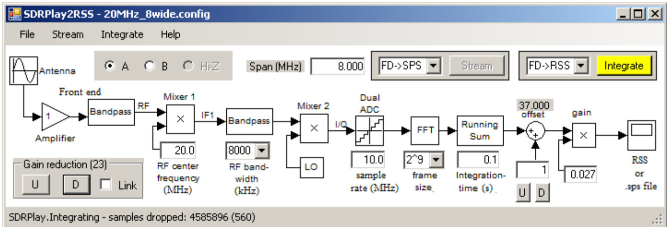
Illustration 38: SDRPlay2RSS application. The yellow Integrate button indicates the active connection with the SDRPlay receiver.
