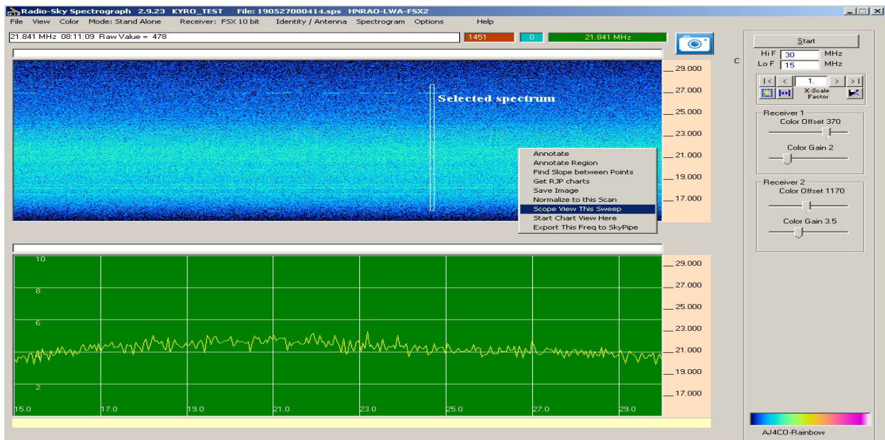
Illustration 7: The Scope View displays the spectrum in a format analogous to a traditional spectrum analyzer.
