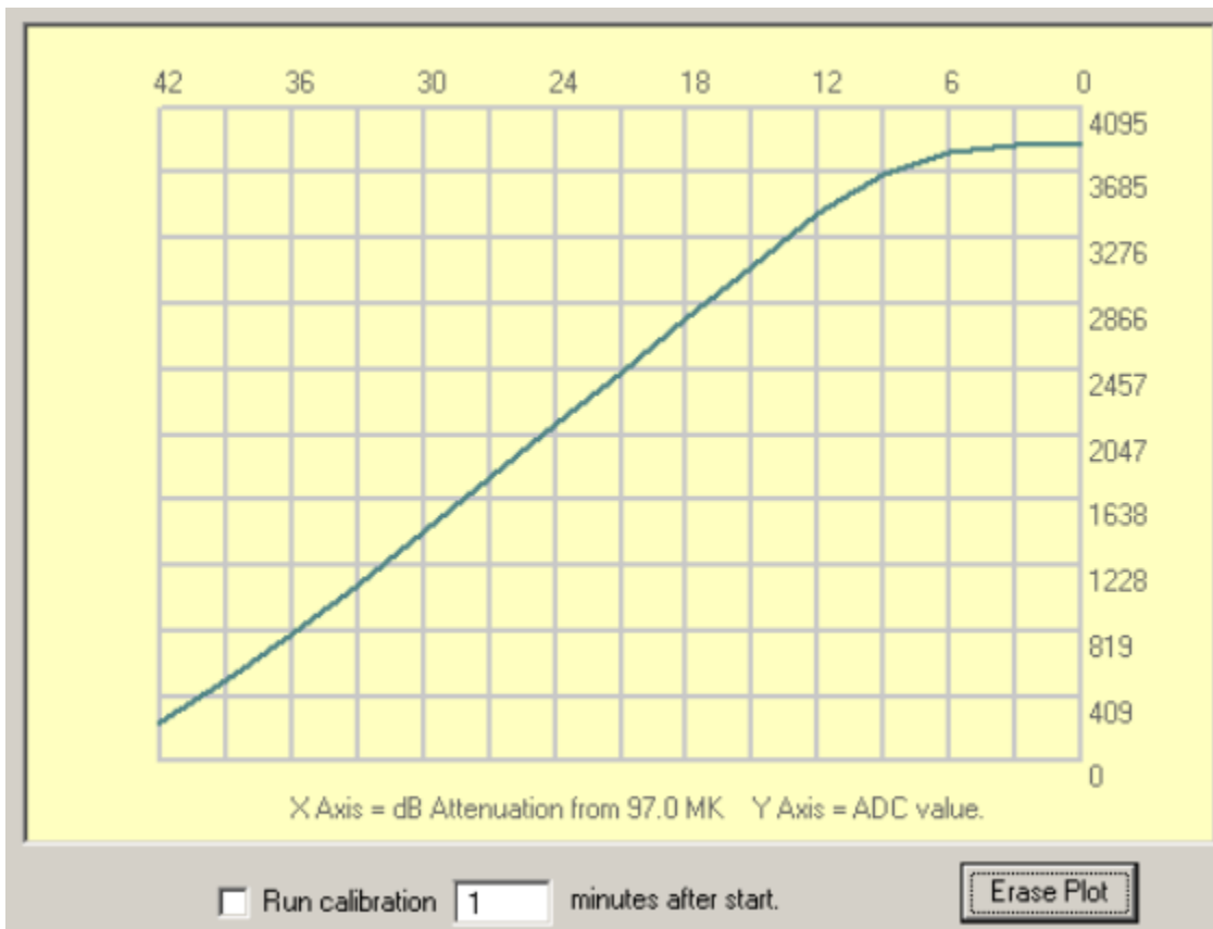
Illustration 26: Plot window from the Calibrator Control panel. In this plot we can see that gain compression is occurring at the higher noise levels.
