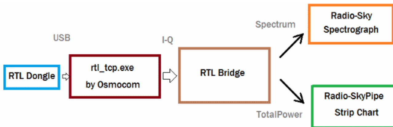
Illustration 34: Diagram of data flow when using RTL Bridge.
